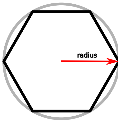
Figure 384: The outer circle of a hexagon
